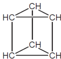
Ladenburg structure
