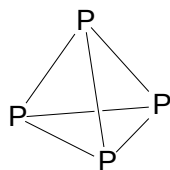
'white' phosphorus
