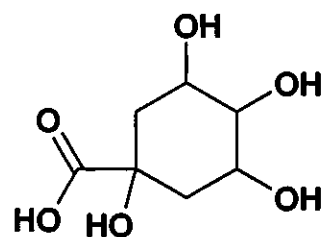
Compound Y
