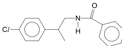
compound V
