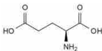
glutamic acid
