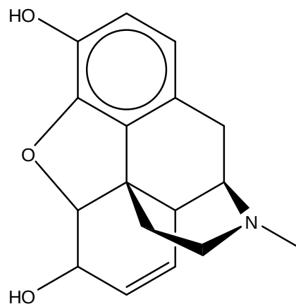
Morphine
