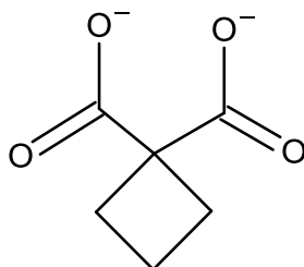
cyclobutanedicarboxylate ion
