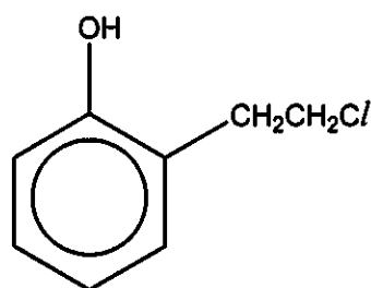
compound X
