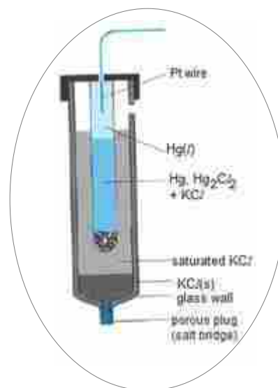
Figure 1: Set-up for potentiometric titration
