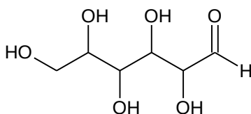
D-glucose
