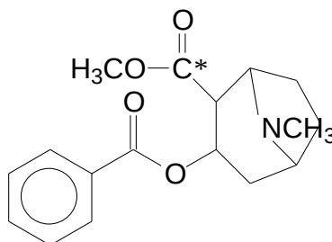
cocaine
