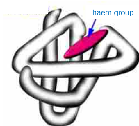
Myoglobin
