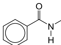
Compound X
