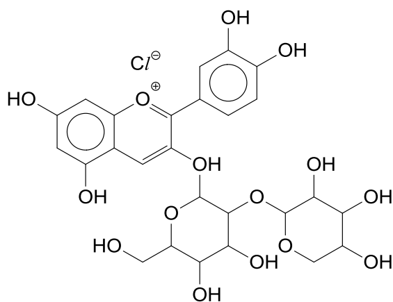
cyanidin 3-sambubioside
