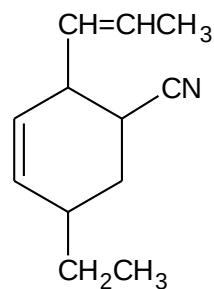
compound P
