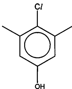
chloroxylenol
