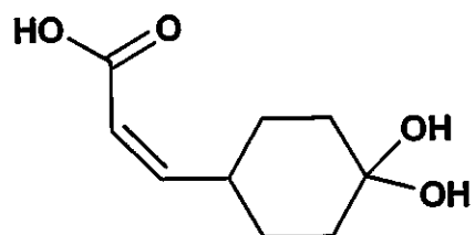
Compound Z
