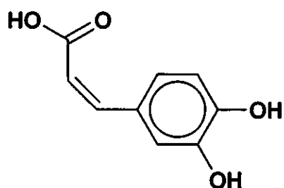
Compound X
