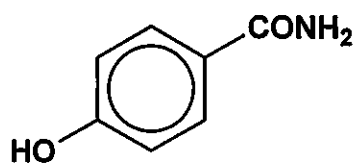
Compound A
