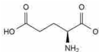
glutamate
