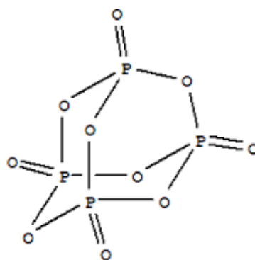
Structure of \text{P}_4\text{O}_{10}
