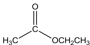
ethyl ethanoate
