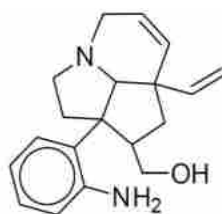
compound X
