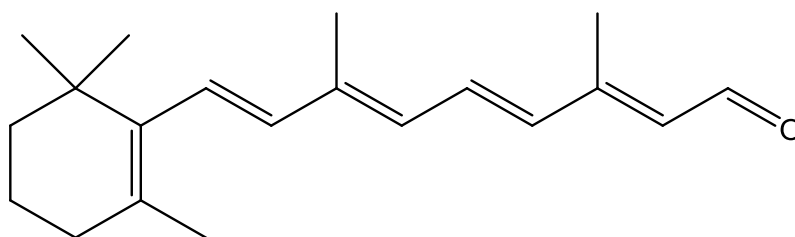
retinal
