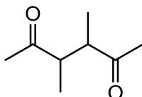
Compound X
