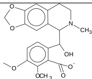
basic conditions
