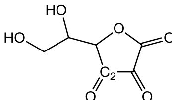
dehydroascorbic acid
