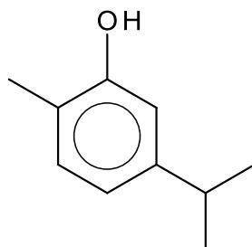
thymol
