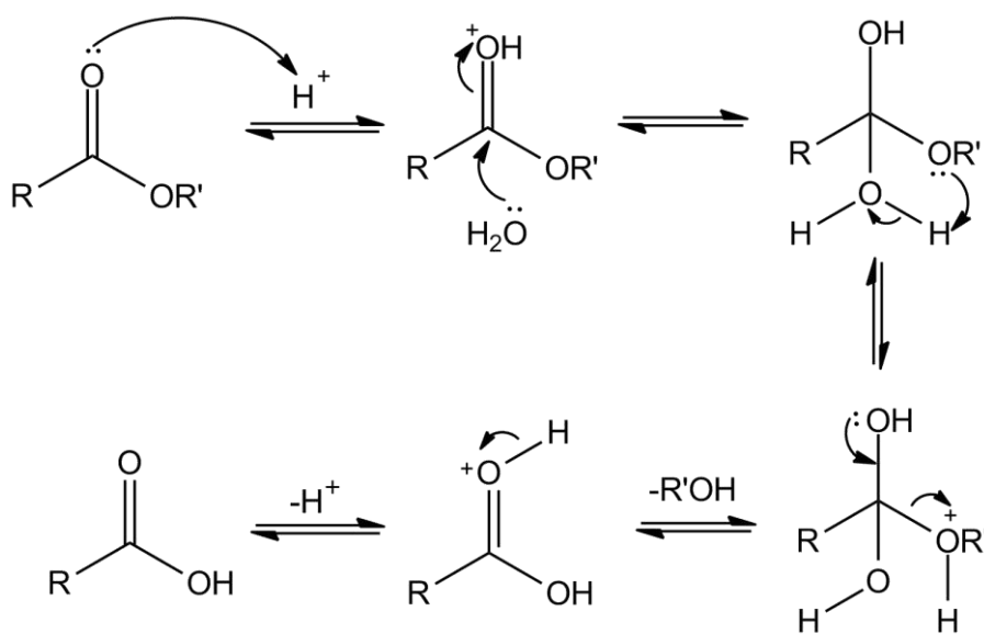
acidic hydrolysis
