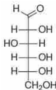
glucose
