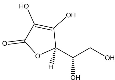
ascorbic acid
