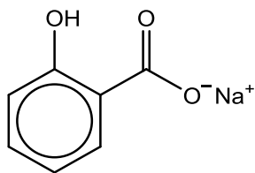
sodium salicylate
