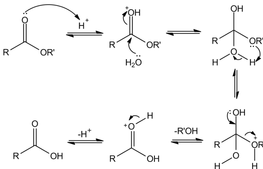
acidic hydrolysis
