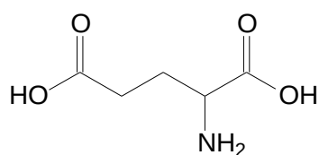
glutamic acid
