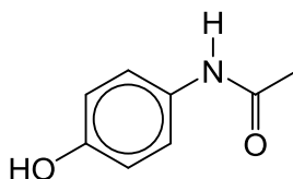
Paracetamol
