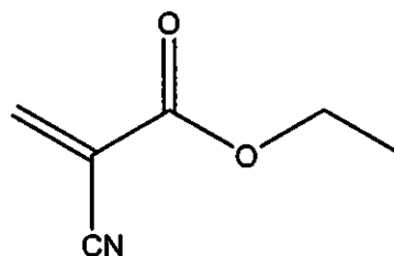
ethyl cyanoacrylate
