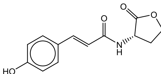
4-coumaroyl-HSL
