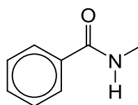
Compound X
